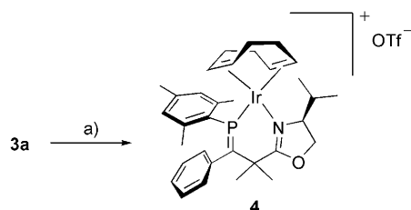
Scheme 3. Synthesis of iridium complex 4 . a) [(cod)IrCl] 2 , AgOTf, CH 2 Cl 2 , RT, 30 min (72%). cod = 1,5-cyclooctadiene, OTf = trifluoromethanesulfonate.
